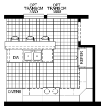
OPTIONAL KITCHEN WITH OVEN STACK
