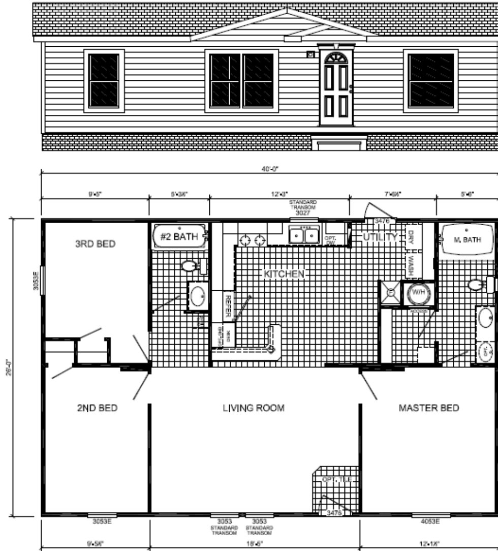
L-2403A 3-BEDROOM / 2-BATH 28 x 44 - Approx. 1040 Sq. Ft.
