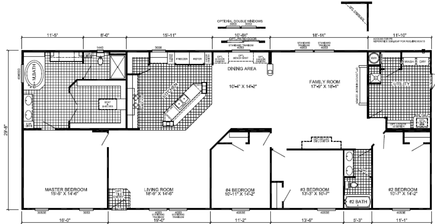
L-3764A 4-BEDROOM / 2-BATH 32 X 80 - Approx. 2254 Sq. Ft.
